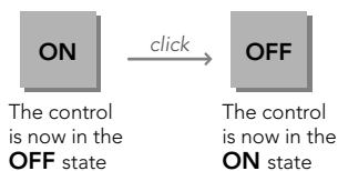
Figure 21-5 Flip-flop button controls are very efficient. They save space by controlling two mutually exclusive options with a single control. The problem with flip-flop controls is that they fail to fulfill the second duty of every control — to inform users of their current state. If the button says ON when the state is off, it is unclear what the setting is. If it says OFF when the state is off, however, where is the ON button? Don't use them.
