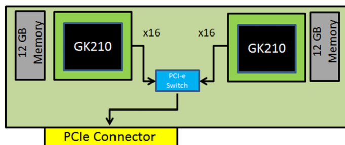
Tesla K80 Block Diagram
