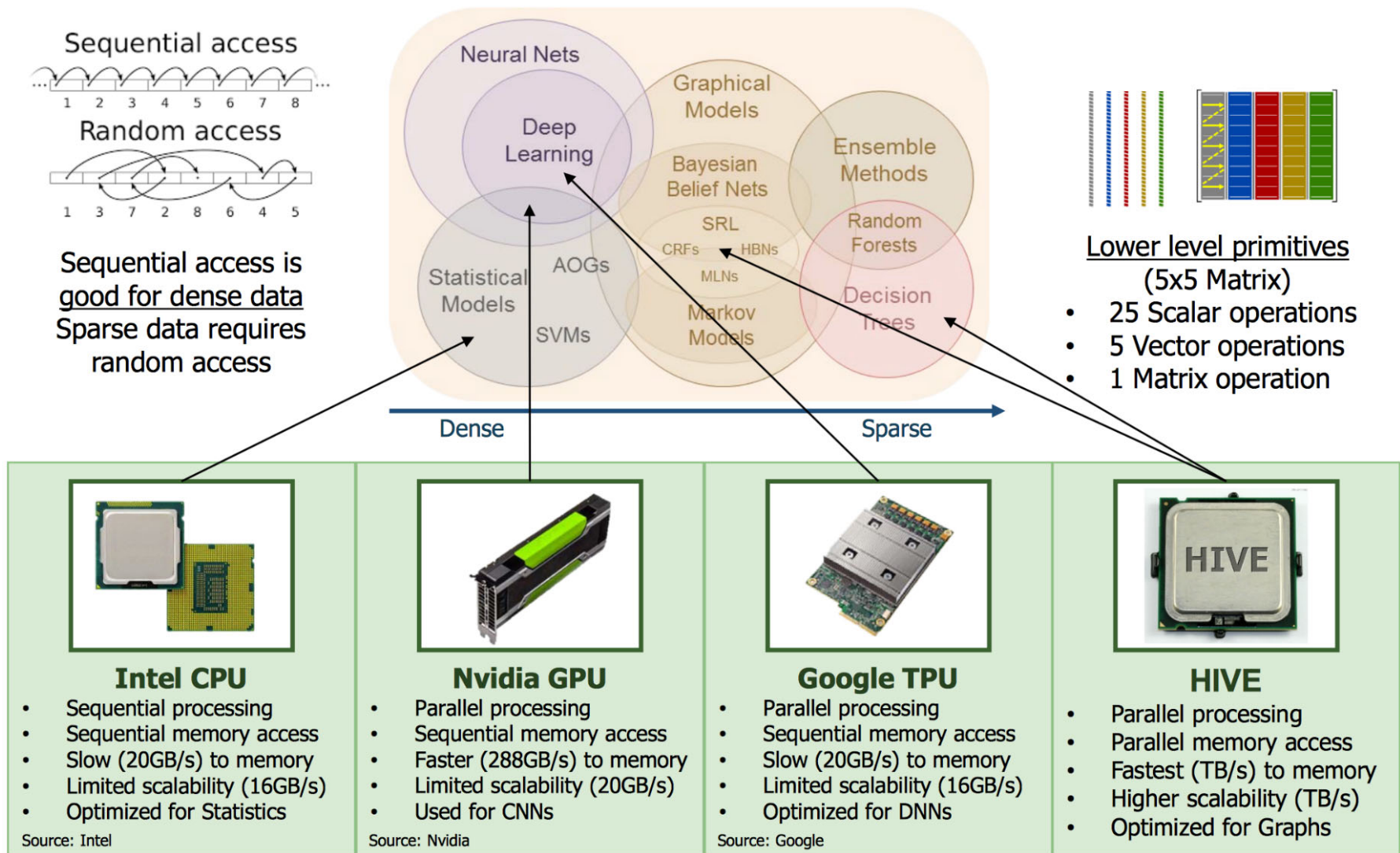
Applications (top) and performance (bottom) comparisons between Intel CPUs, Nvidia GPUs, Google TPUs, and DARPA's proposed HIVE processor. (Source: DARPA)
