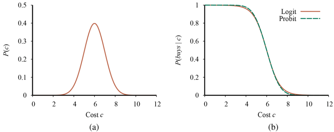
(a) A normal (Gaussian) distribution for the cost threshold, centered on \mu = 6.0 with standard deviation \sigma = 1.0 . (b) Expit and probit models for the probability of buys given cost , for the parameters \mu = 6.0 and \sigma = 1.0 .
