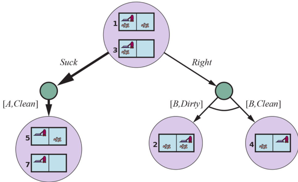
The first level of the AND-OR search tree for a problem in the local-sensing vacuum world; Suck is the first action in the solution.
