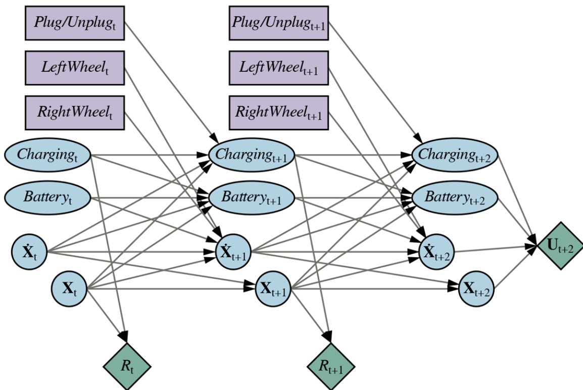
A dynamic decision network for a mobile robot with state variables for battery level, charging status, location, and velocity, and action variables for the left and right wheel motors and for charging.
