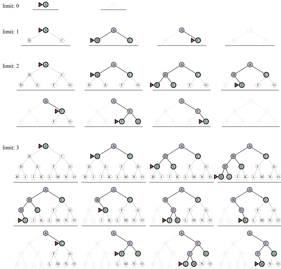
Four iterations of iterative deepening search for goal M on a binary tree, with the depth limit varying from 0 to 3. Note the interior nodes form a single path. The triangle marks the node to expand next; green nodes with dark outlines are on the frontier; the very faint nodes provably can't be part of a solution with this depth limit.
