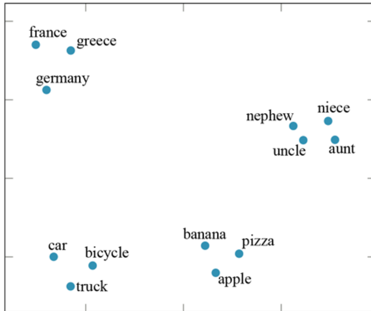
Word embedding vectors computed by the GloVe algorithm trained on 6 billion words of text. 100-dimensional word vectors are projected down onto two dimensions in this visualization. Similar words appear near each other.
