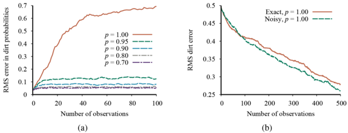
(a) Performance of the standard particle filtering algorithm with 1,000 particles, showing RMS error in marginal dirt probabilities compared to exact inference for different values of the dirt persistence p . (b) Performance of Rao-Blackwellized particle filtering (100 particles) compared to ground truth, for both exact location sensing and noisy wall sensing and with deterministic dirt. Data averaged over 20 runs.
